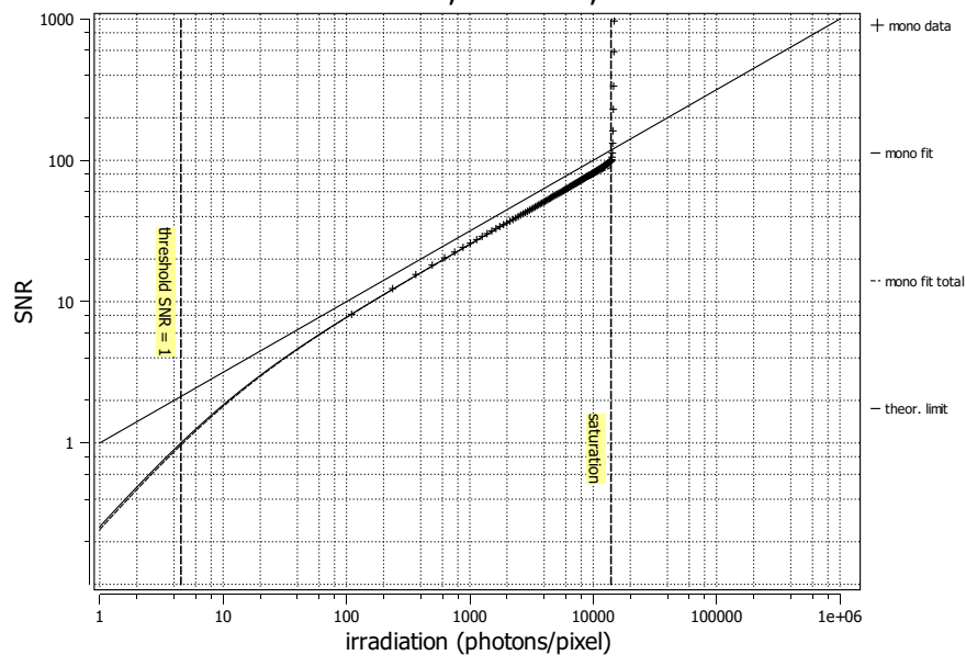
SNR mACC300098, 533 nm, 26.04.2023
