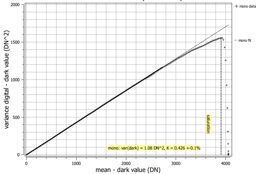
Photon transfer mACC300098, 533 nm, 26.04.2023
