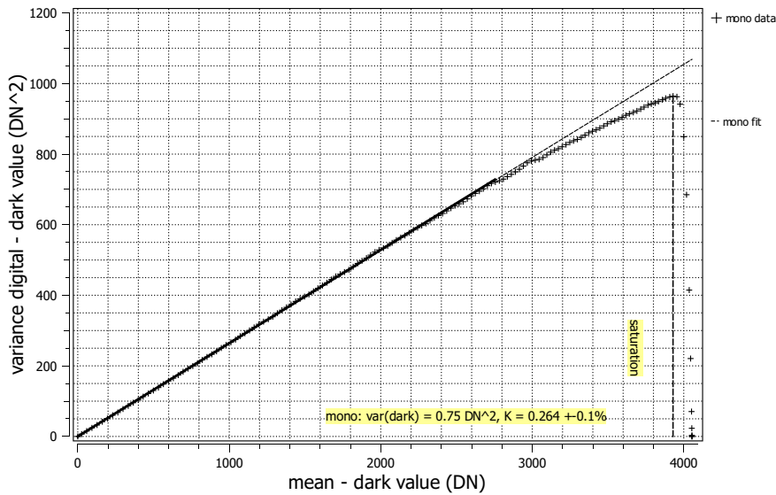
Photon transfer m_ACC3_00021, 533 nm, 06.03.2023
