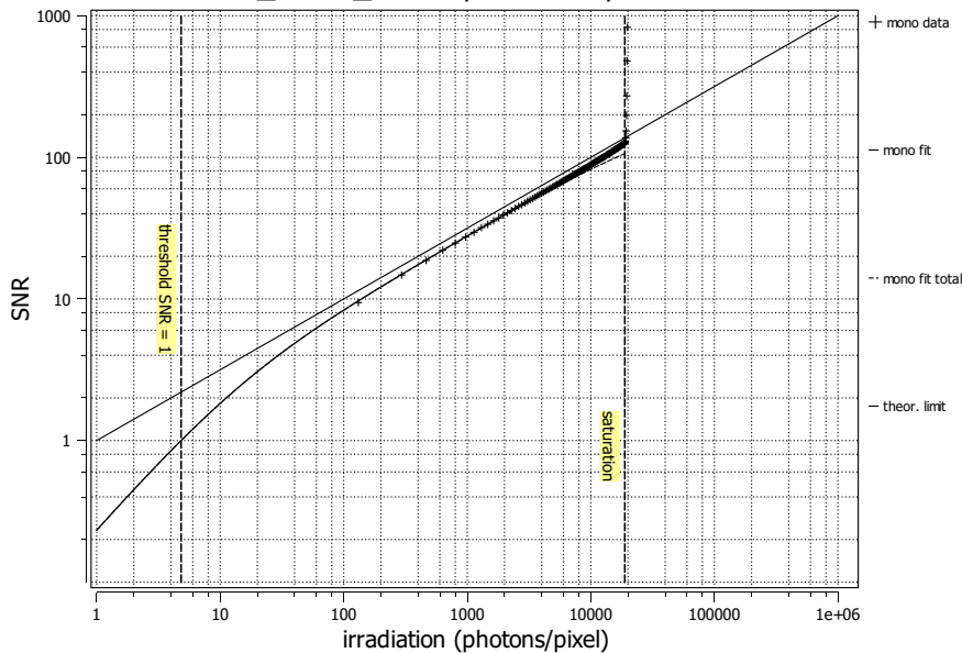
SNR m_ACC3_00021, 533 nm, 06.03.2023
