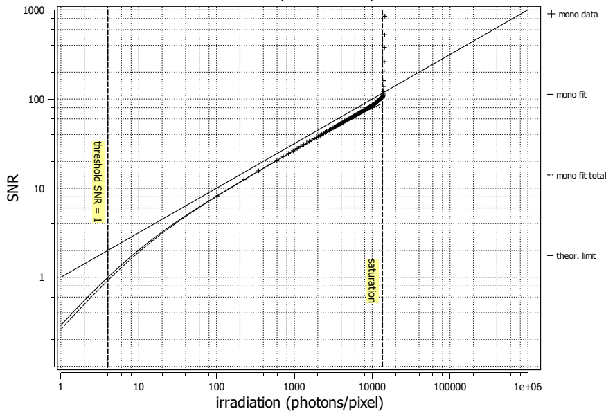
SNR mACC300128, 533 nm, 08.05.2023
