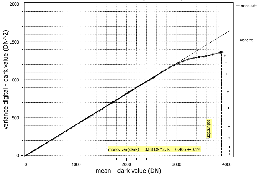
Photon transfer mACC300128, 533 nm, 08.05.2023
