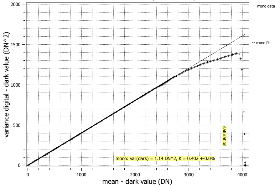
Photon transfer mACC300142, 533 nm, 16.05.2023
