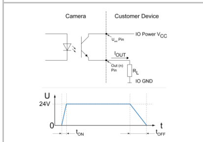
Digital Output: High Active
