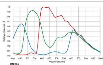
Sensor Graph: Relative Response
